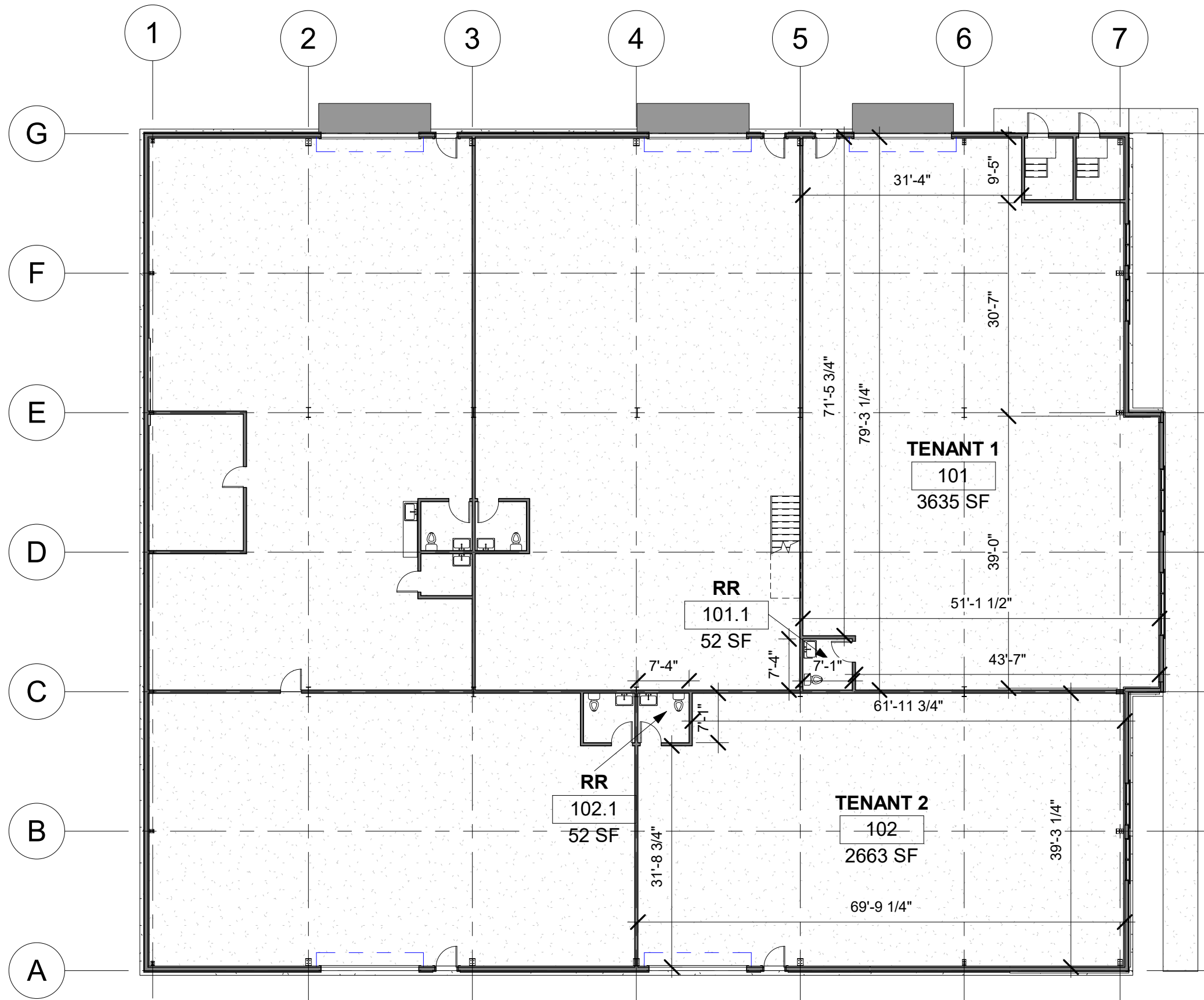
1 1ST FL PLAN - M 1/16" = 1'-0"
